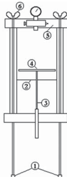
Figure 2 Pressure-chamber: 1 – rotatable feet, 2 – fluid level, 3 and 4 – height adjustable base for carrying specimens, 5 – Plexiglas lid, 6 – wing nuts
